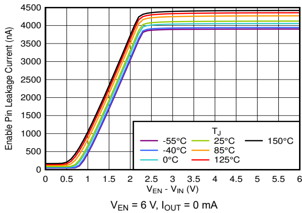
Figure 6-43. Enable Pin Leakage Current vs V_{EN} - V_{IN} V_{EN} = 6 \text{ V} , I_{OUT} = 0 \text{ mA}
