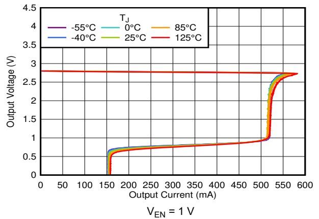
Figure 6-44. Current Limit V_{EN} = 1 \text{ V}
