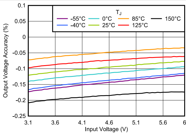
Figure 6-21. Output Voltage Accuracy vs V_{IN}
