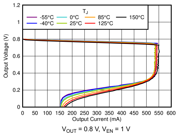
Figure 6-45. Current Limit V_{OUT} = 0.8 \text{ V} , V_{EN} = 1 \text{ V}
