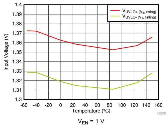
Figure 6-46. UVLO Threshold vs Temperature V_{EN} = 1 \text{ V}
